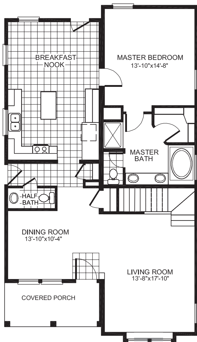
FIRST FLOOR (1,320 sq. ft.)
