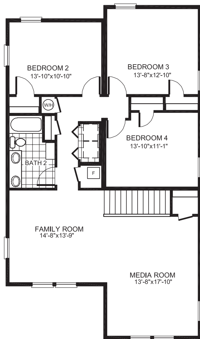
SECOND FLOOR (1,320 sq. ft.)
